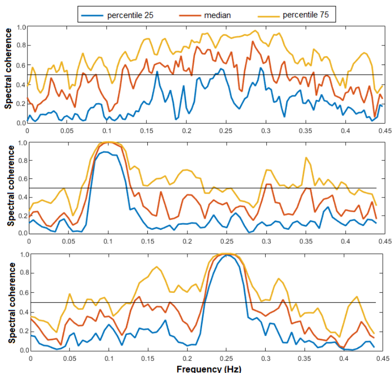
Figure 2 Results of the spectral coherence analysis between HRV and AR in 12 healthy subjects during spontaneous breathing (upper panel), controlled breathing at 0.1 Hz (middle panel) and controlled breathing at 0.25 Hz (lower panel). All recordings were obtained during supine position.
