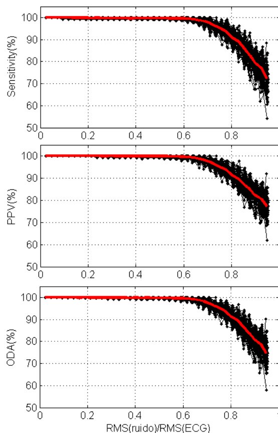
Figure 1 Performance of QRS detection algorithm in 100 tests with simulated ECG and additive noise. Black lines = individual tests, red line = mean from all tests.
